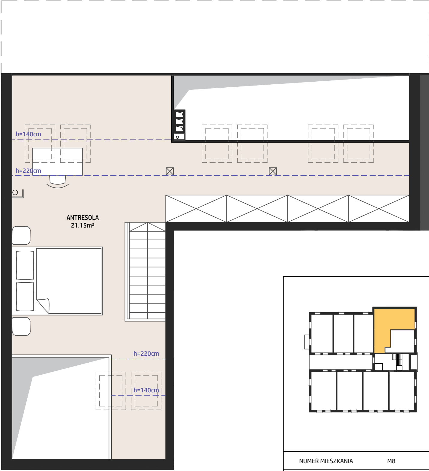
PODDASZE: 21,15m²
